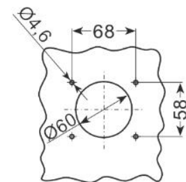
Montering termostat
